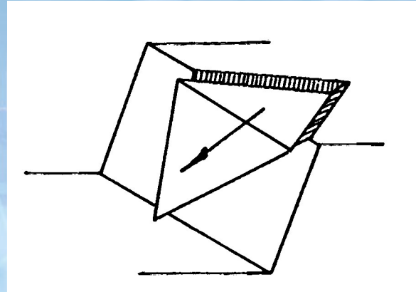
Wedge Failure
