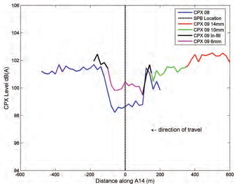
Figure 4.1: CPX results Creeping St. Mary '08 and '09, 80 km / h
