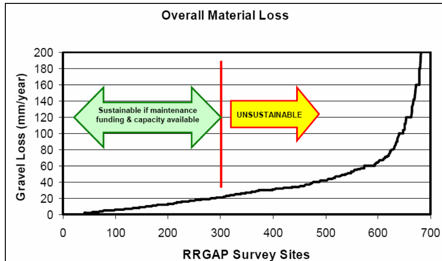
Figure 2.2: Material Loss Summary of the Vietnam Experiment (Petts. et. al, 2005)
