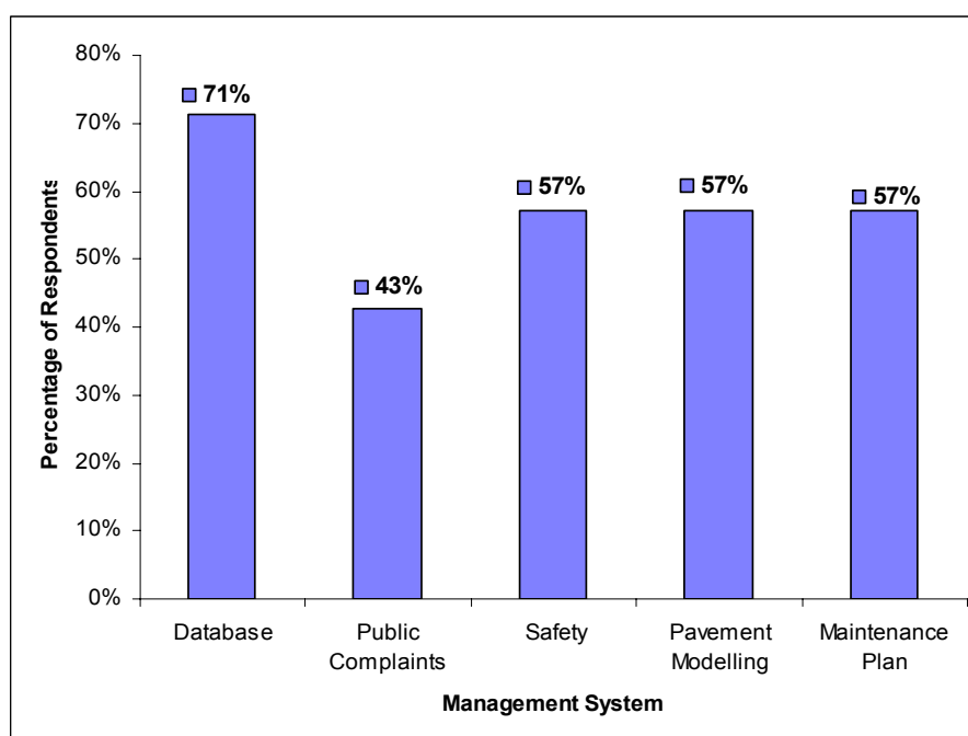
Figure D.7.2: Systems Used for Managing Unsealed Roads
