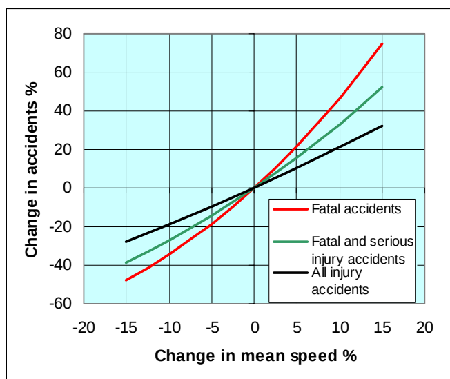
Figure 2.4. The power model: relationship between change in mean speed and accidents
