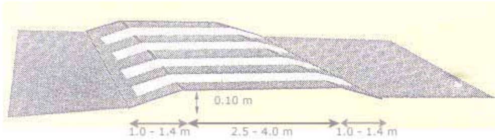
Figure 4.7. Hump at a pedestrian crossing 15
