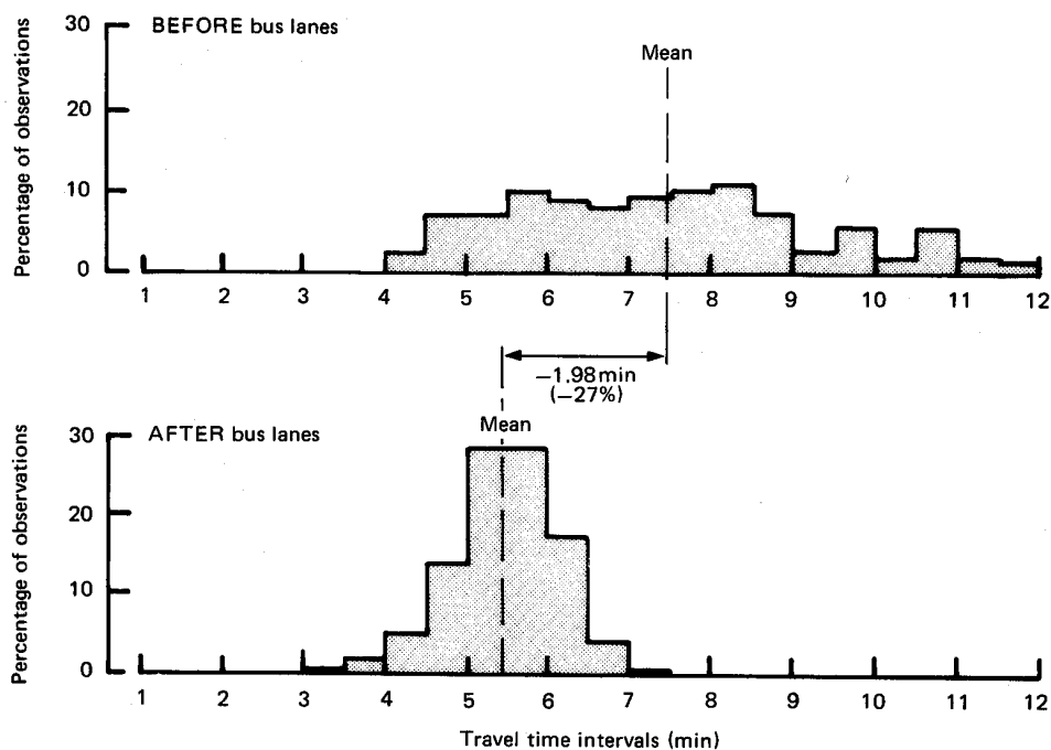
Fig. 5.1 Bus travel time changes, Paholyothin Road
