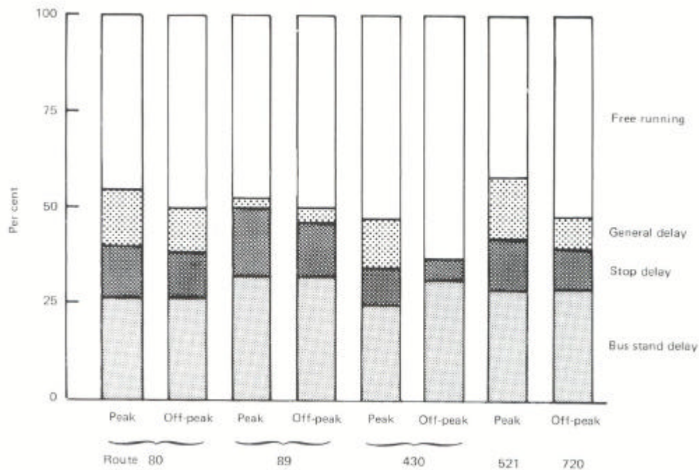
Fig. 3.3 Examples of a breakdown of bus running times
