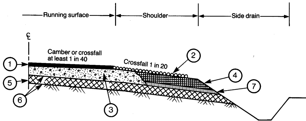
(a) Separate shoulder material
