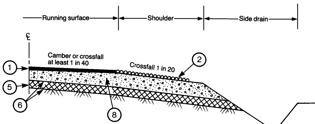
(b) Extended roadbase and sub-base
