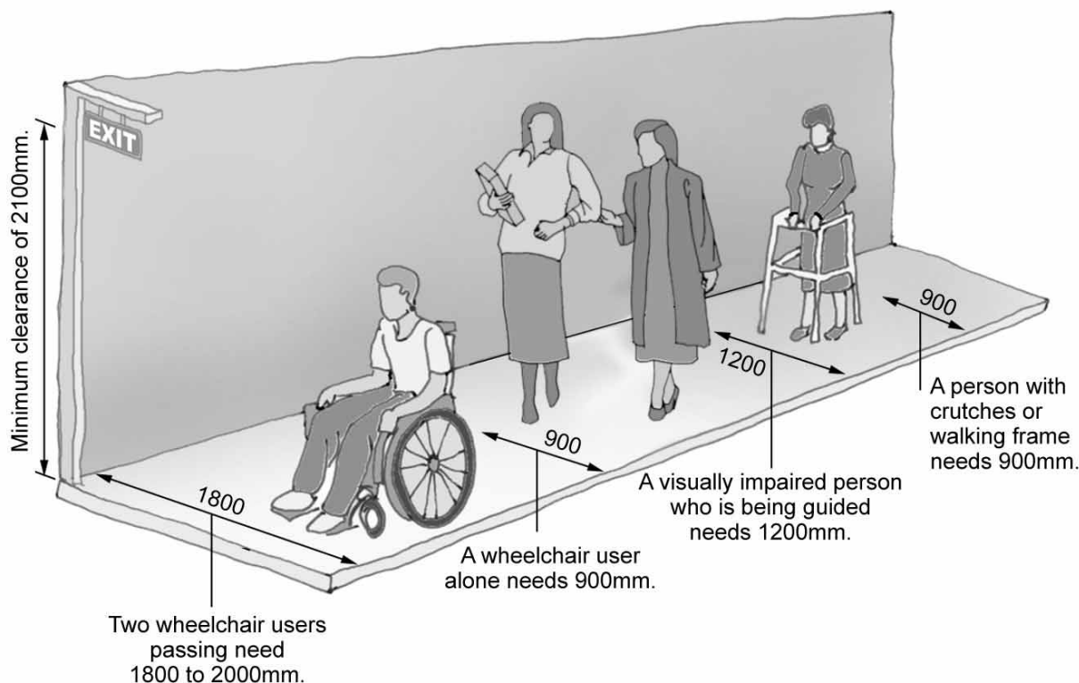
Figure 3.7 Minimum dimensions for walkways (Adapted from Oxley, 2002)
