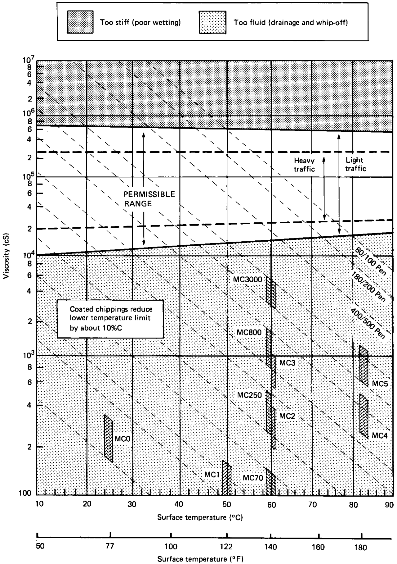
Fig.15 Surface temperature/choice of binder for surface dressing
