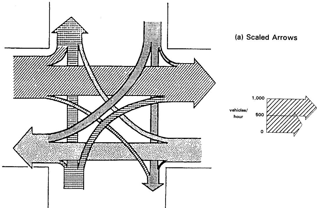
Figure 6.2 Presentation of Junction Count Surveys
