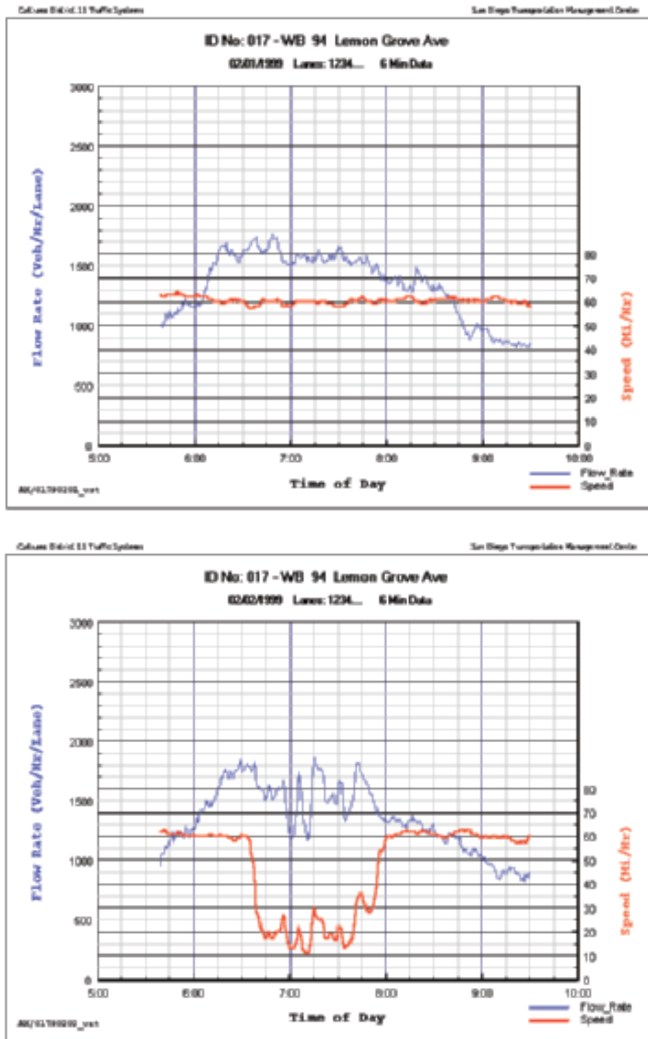
Figure 9.1. Access Control: Ramp-Metering, impacts on Traffic Volume and Speed in San Diego, California
