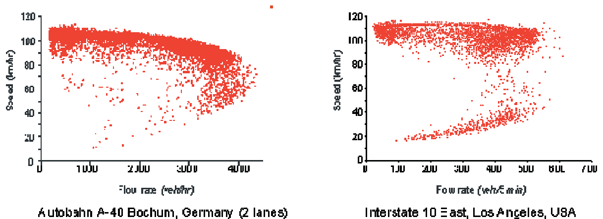
Figure 3.5. Speed-Flow Curves for Two Urban Motorways
