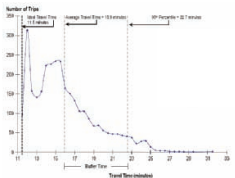
Figure 2.2. Distribution of Travel Times: State Route 520 Seattle, Eastbound, 4:00-7:00 p.m. Weekdays (11.5 Miles Long)
