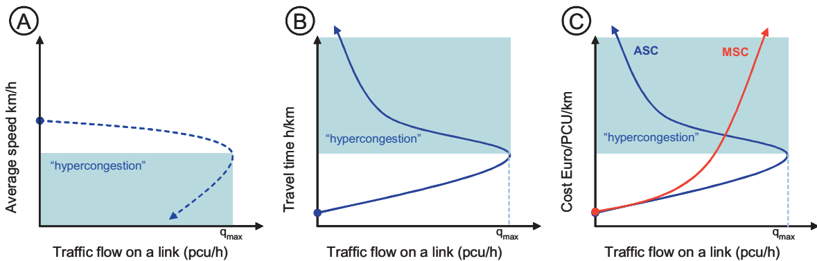
Figure 5.2. Translation of the Fundamental Speed-Flow Diagram into a Cost Function
