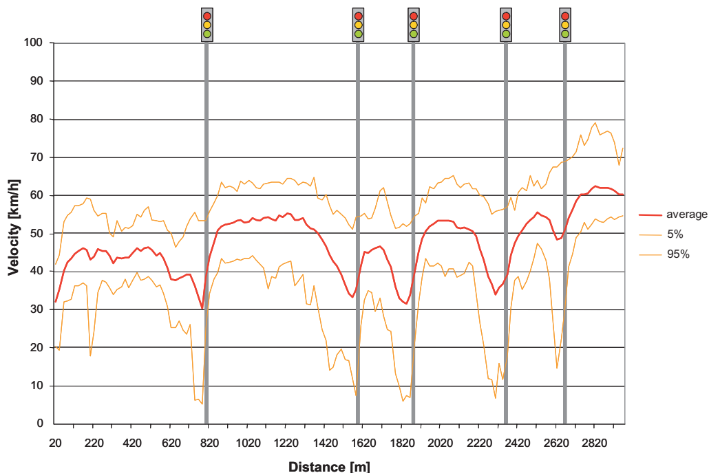
Figure 3.8. Aggregated Floating Car Data for a Section of a Signalized 2-lane Major-Road in Munich
