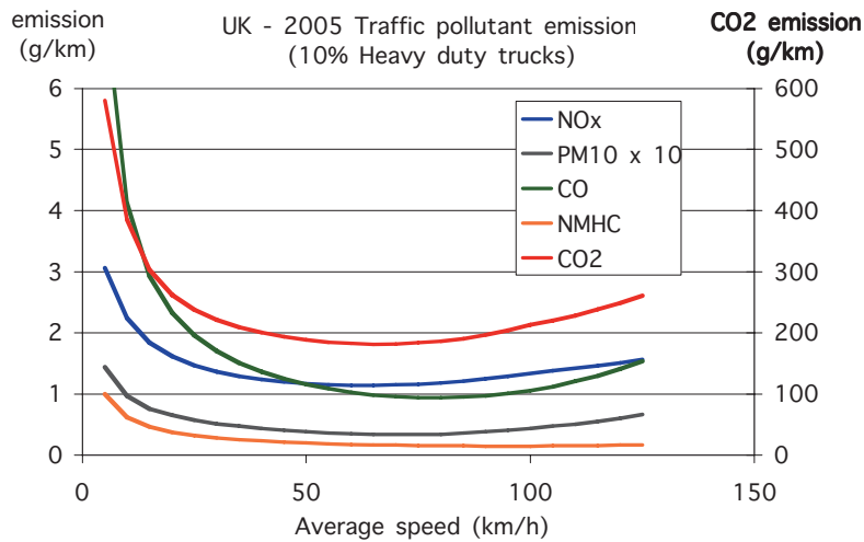
Figure 5.12. Traffic Emissions vs. Average Speed (UK DfT)
