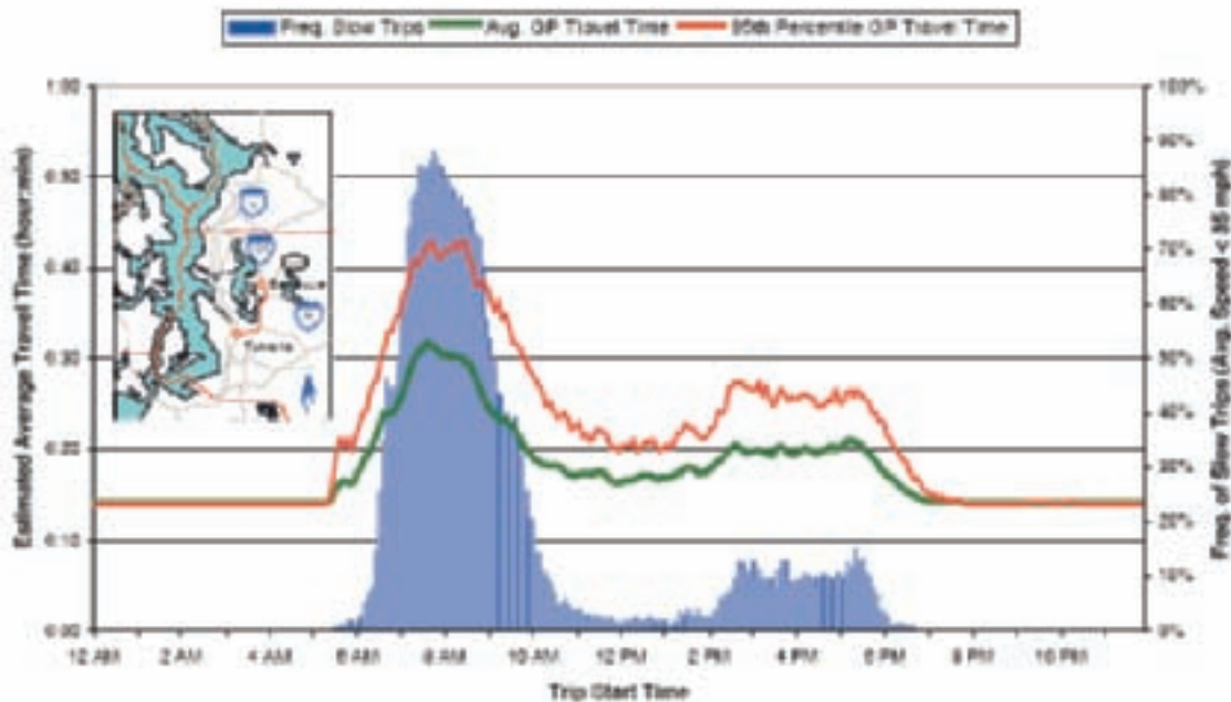
Figure 2.6. Estimated Average, 95th Percentile Travel Times and Frequency of Heavy Congestion 2003: Tukwila to Bellevue CBD via I-405 (General Purpose Lanes - 13.8 miles)
