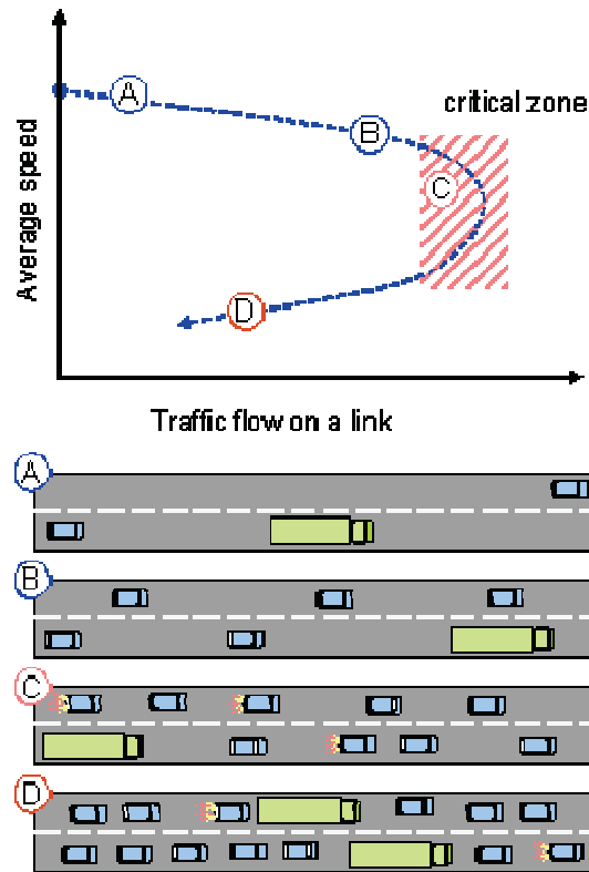
Figure 3.4. Uninterrupted Flow Speed-Flow Curve
