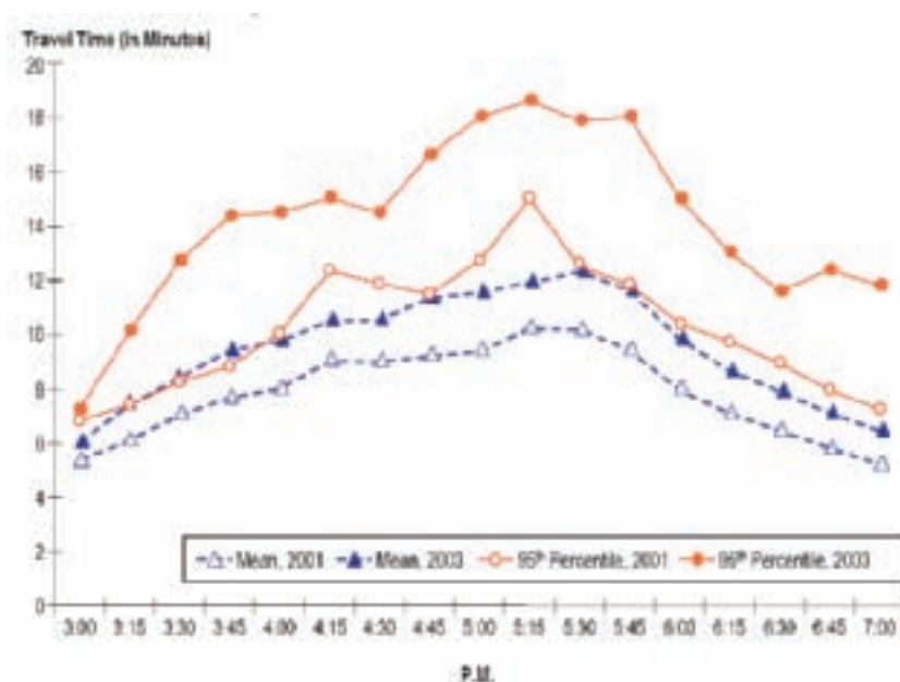
Figure 2.4. Travel Time Index, Planning Time and Buffer Index: I-95 Atlanta
