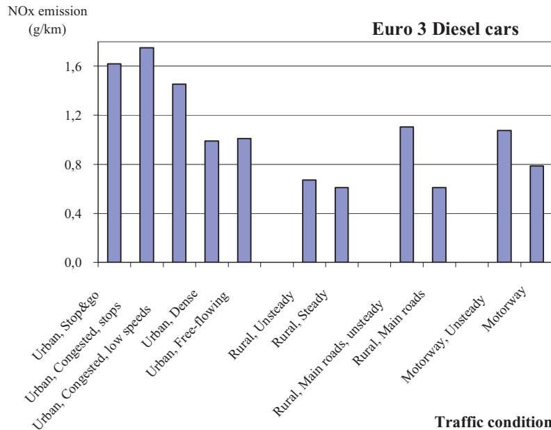
Figure 5.13. Influence of Different Traffic Conditions on the Pollutant Emissions (ARTEMIS Research Project)
