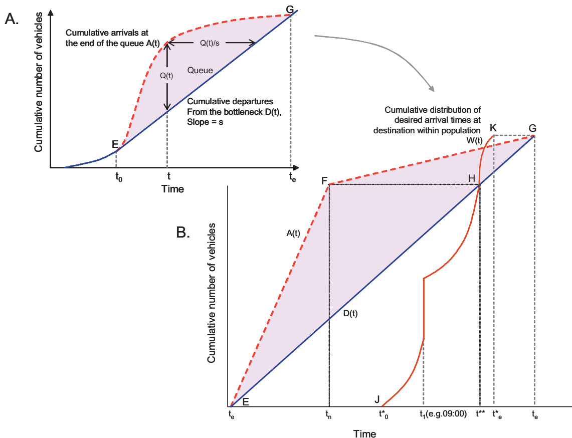
Figure 5.6. Bottleneck Model: Queue Evolution and Equilibrium Trip Timing
