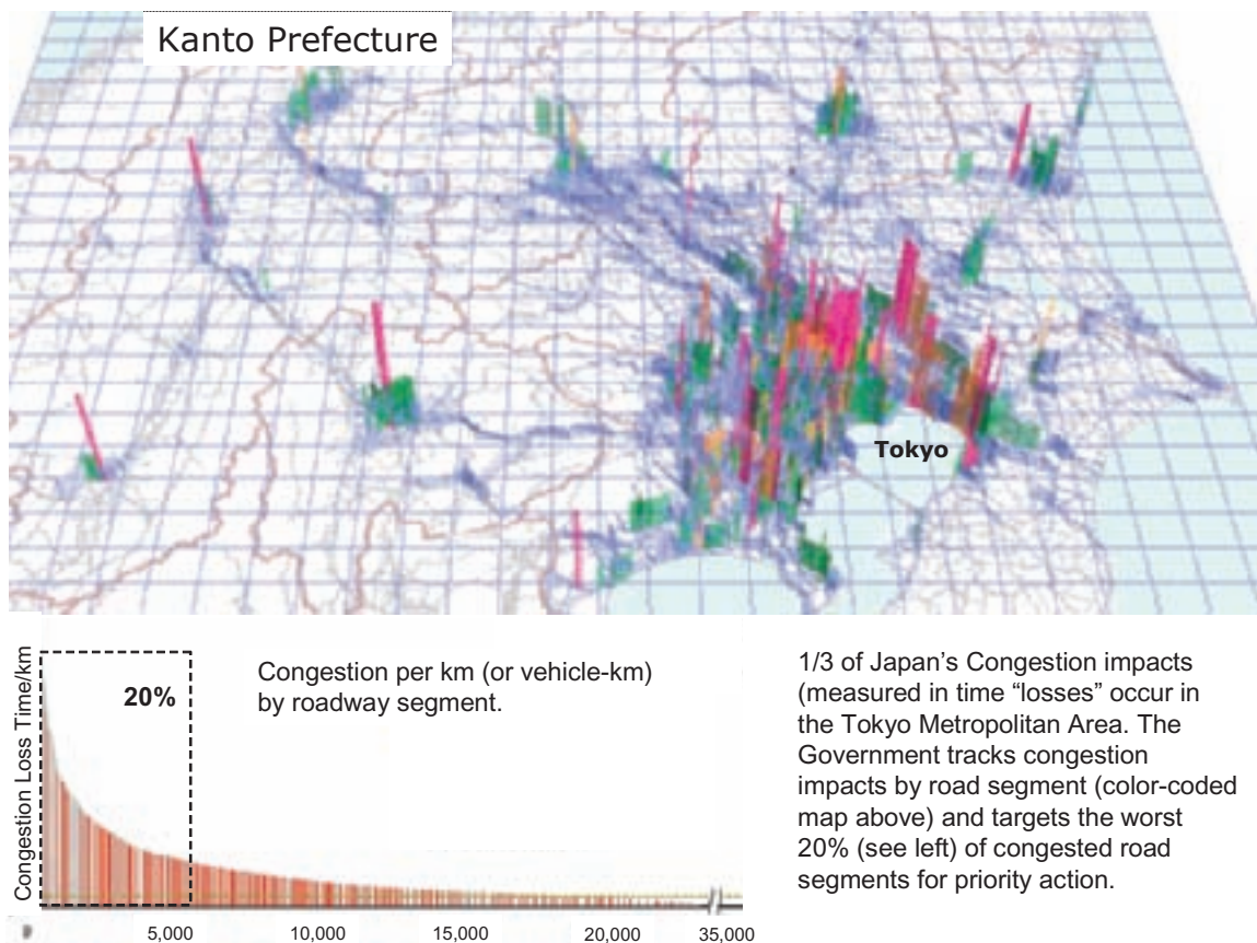
Figure 5.1. Congestion Severity Mapping (time “loss”/km), Kanto Prefecture, Japan
