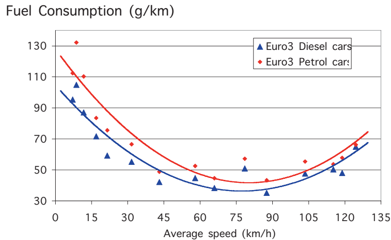
Figure 5.11. Fuel Consumption vs. Average Speed for Recent Diesel and Petrol Cars (ARTEMIS Project)
