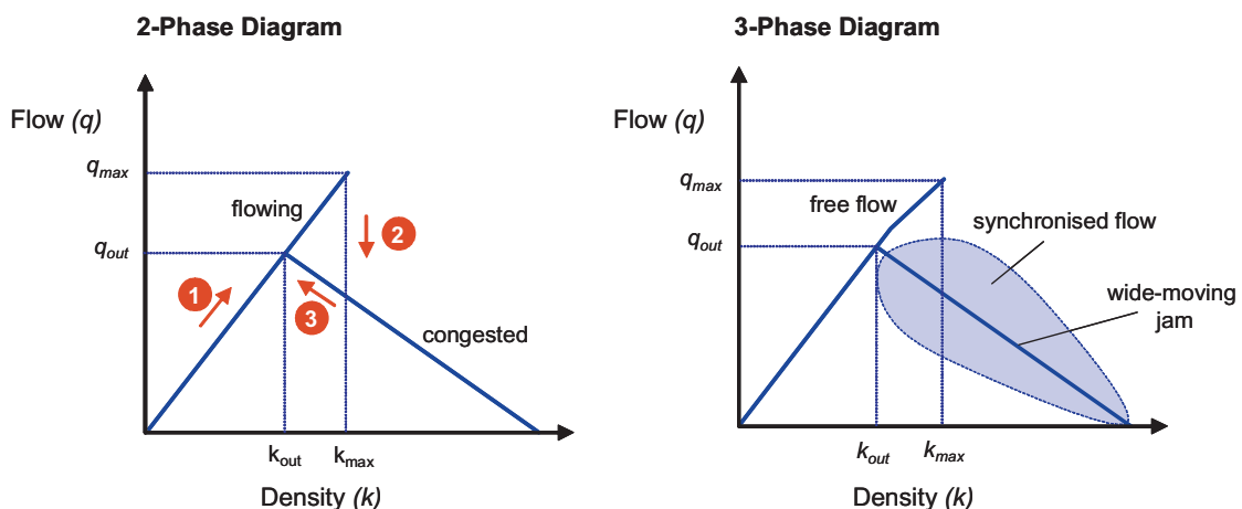
Figure 3.6. Capacity Drop Illustrated for Two-Phase and Three Phase Models
