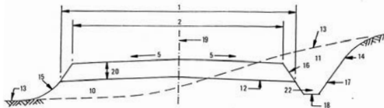
UNPAVED ROAD SECTION
