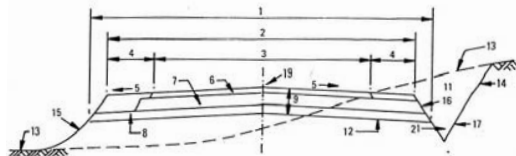
PAVED ROAD SECTION
