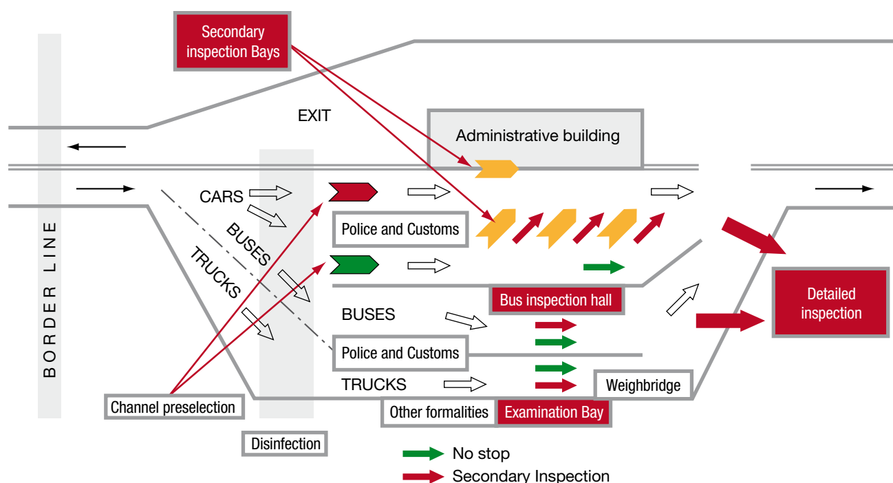
Diagram 6.6 Border crossing point with several linear primary inspection lanes and herringbone vehicle parking bays (World Bank, 2004)
