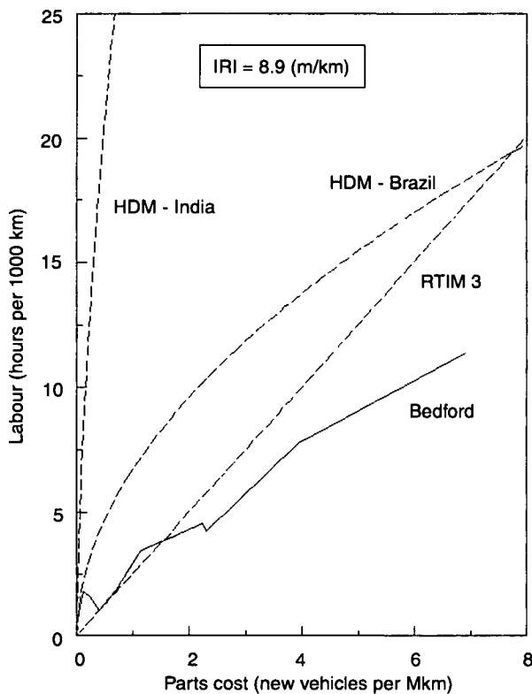
Fig.10 Observed and predicted labour hours - trucks in St Helena
