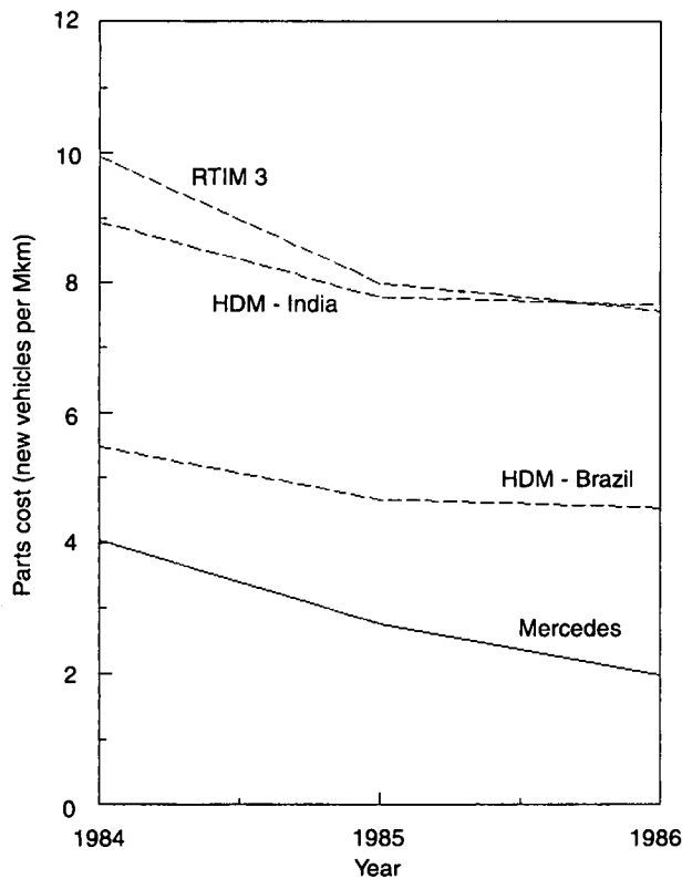
Fig.4 Observed and predicted parts cost - articulated trucks in Botswana
