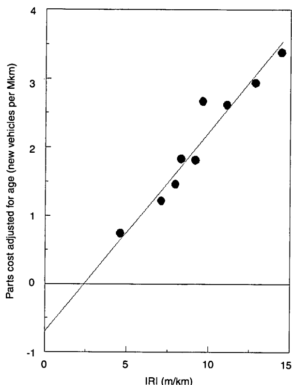
Fig.15 Fitting a simple parts model - articulated trucks in Botswana
