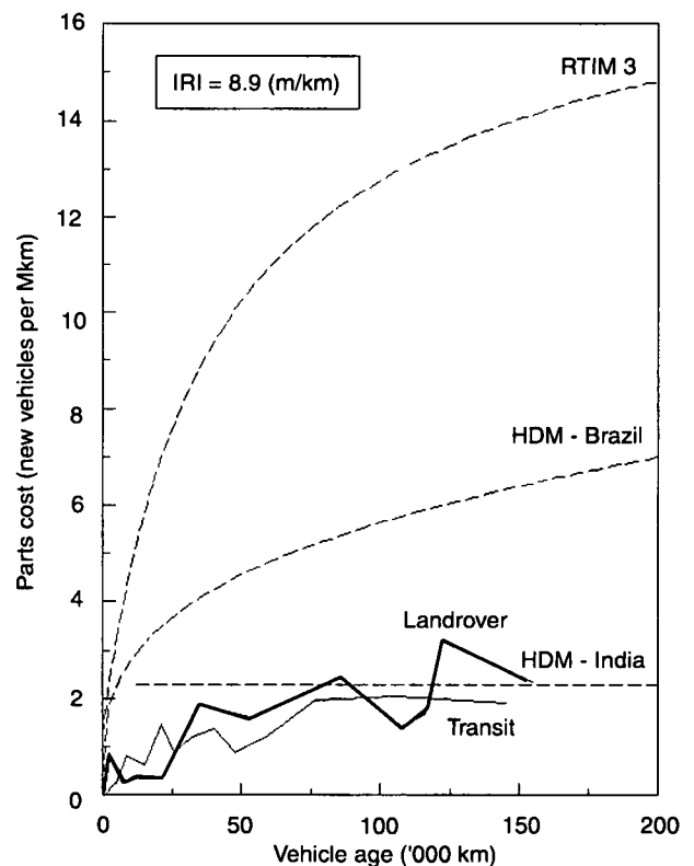
Fig.6 Observed and predicted parts cost - utilities in St Helena
