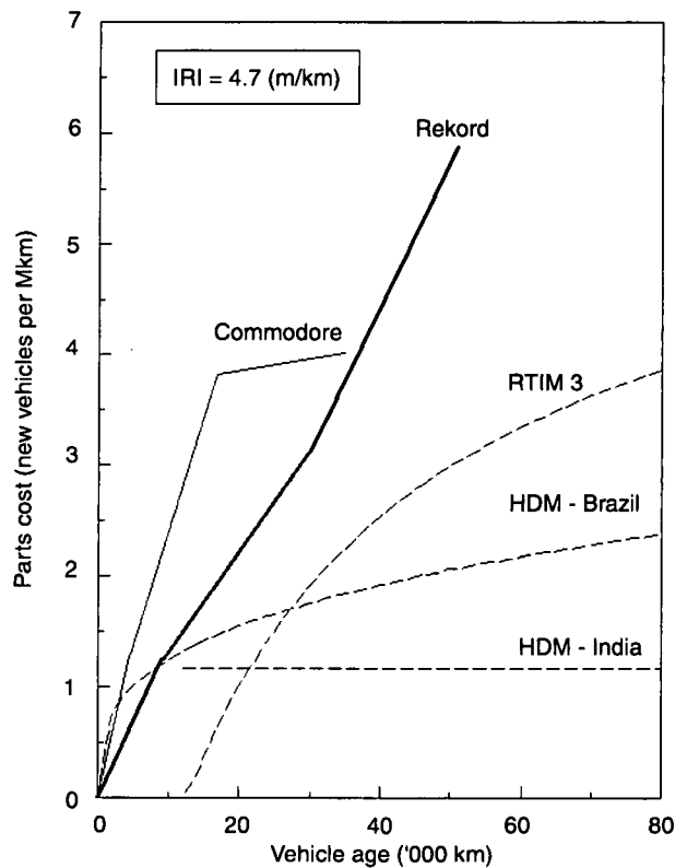
Fig.1 Observed and predicted parts cost - cars in Botswana
