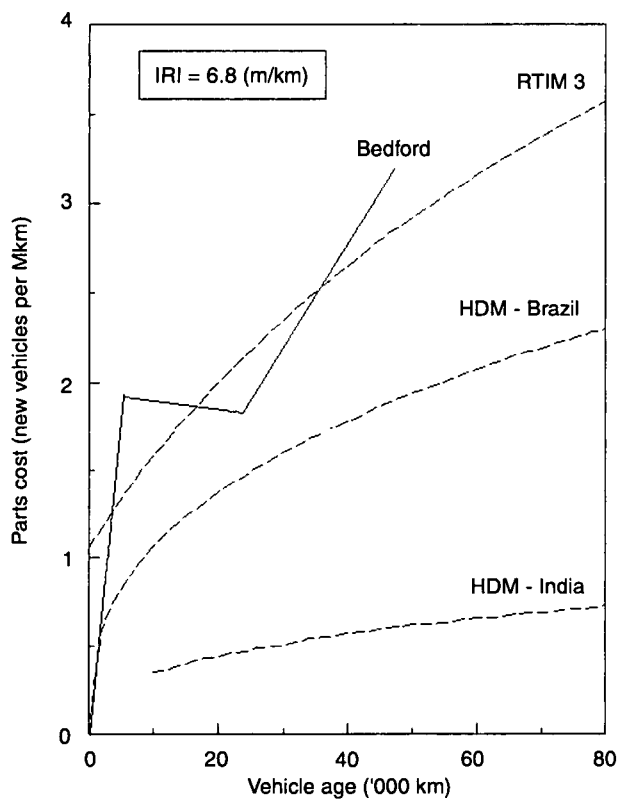
Fig.3 Observed and predicted parts cost - trucks in Botswana
