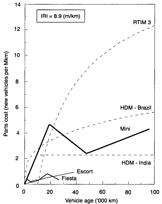
Fig.5 Observed and predicted parts cost - cars in St Helena
