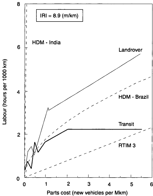
Fig.9 Observed and predicted labour hours - utilities in St Helena
