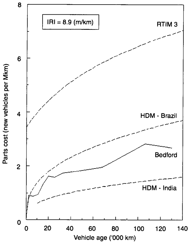
Fig.7 Observed and predicted parts cost - trucks in St Helena
