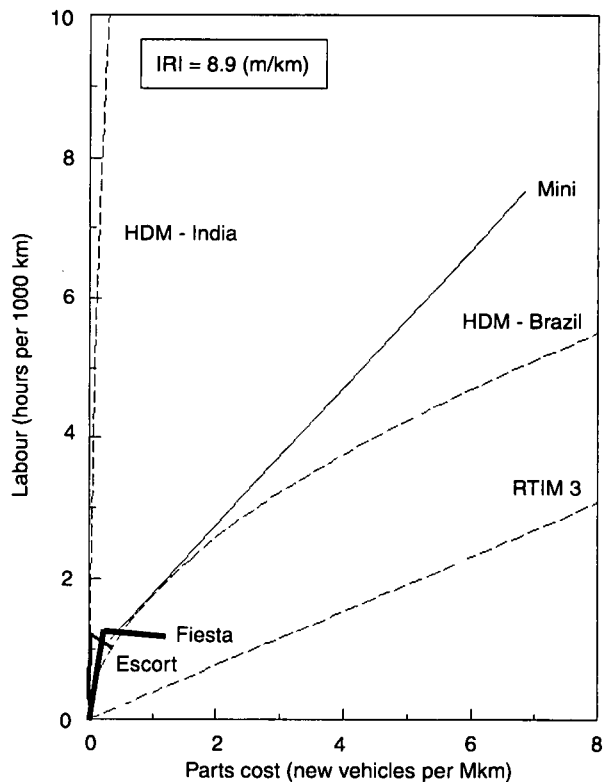
Fig.8 Observed and predicted labour hours - cars in St Helena
