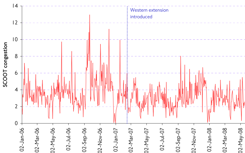
Figure 4.15 SCOOT indicator of 'congestion', links inside the western extension zone at 20 SCOOT equipped junctions around the zone boundary. January 2006–May 2008.
