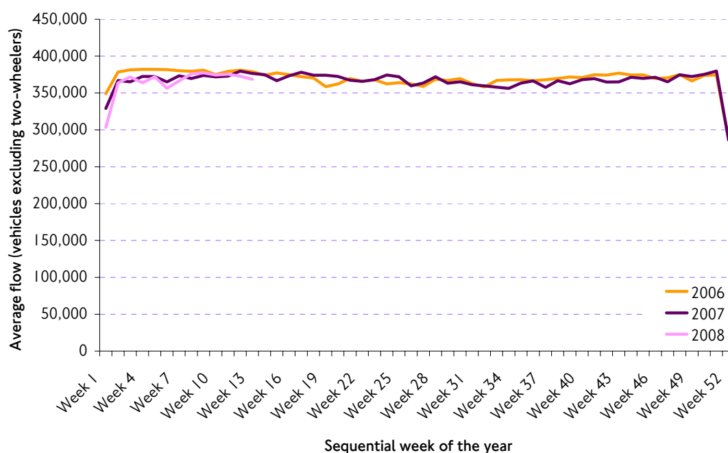
Figure 3.10 Weekly average traffic flows on the Inner Ring Road. Charging hours, 07:00-18:00, 2006 to 2008, vehicles with four or more wheels.
