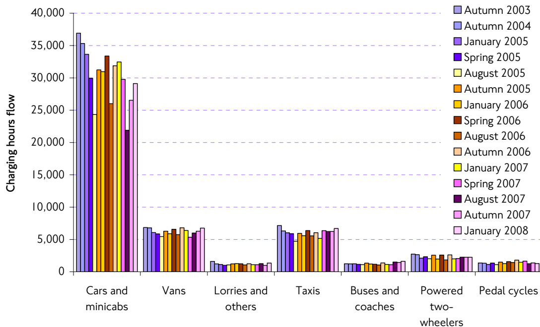
Figure 2.9 Traffic crossing the internal east-west screenline. Both directions combined, by main vehicle type. Charging hours, 07:00–18:00, 2005 to 2007.
