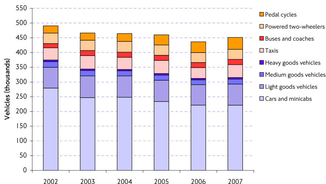
Figure 3.11 Traffic at the central London cordon (extended version wholly outside the original central London charging zone). Inbound direction only, charging hours, 07:00–18.00. Autumn surveys.
